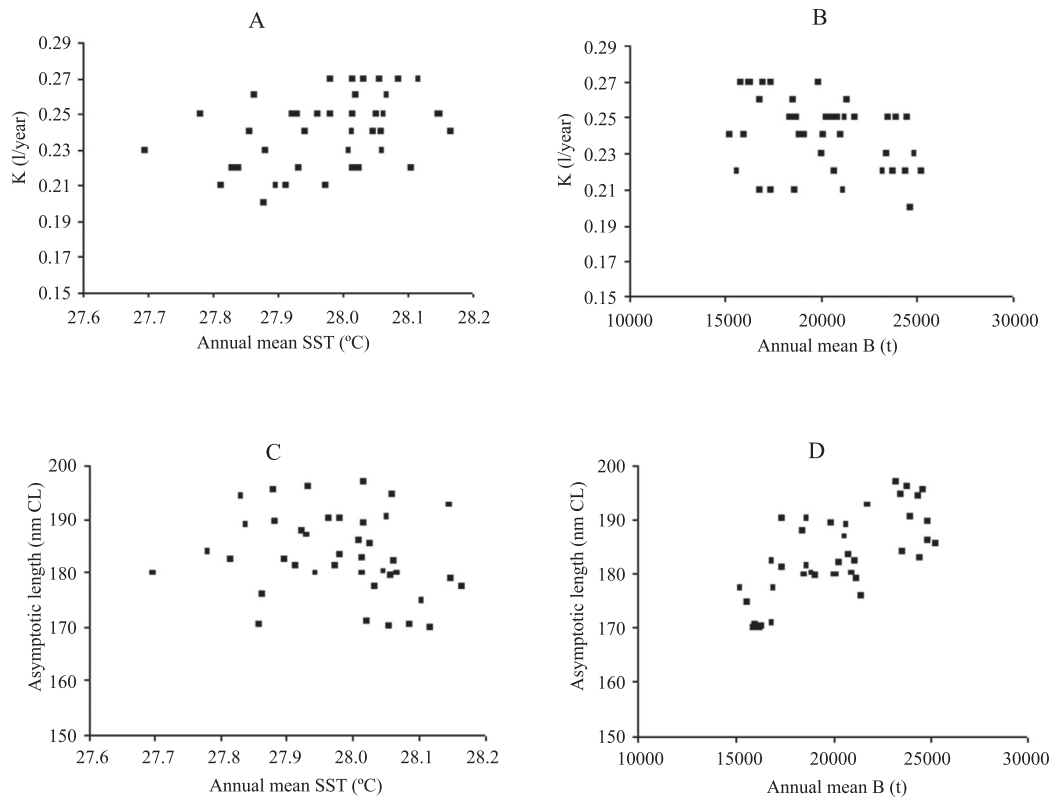
Fig. 4. Plotting raw data of the (A) Annual mean SST (°C) and (B) annual mean biomass (t) versus annual instantaneous growth parameter- K . ( \text{year}^{-1} ) as dependant variable, and the corresponding transformation of (C) annual mean SST and (D) annual mean biomass with the asymptotic length parameter- L_{\infty} (mm CL) as response variable.
