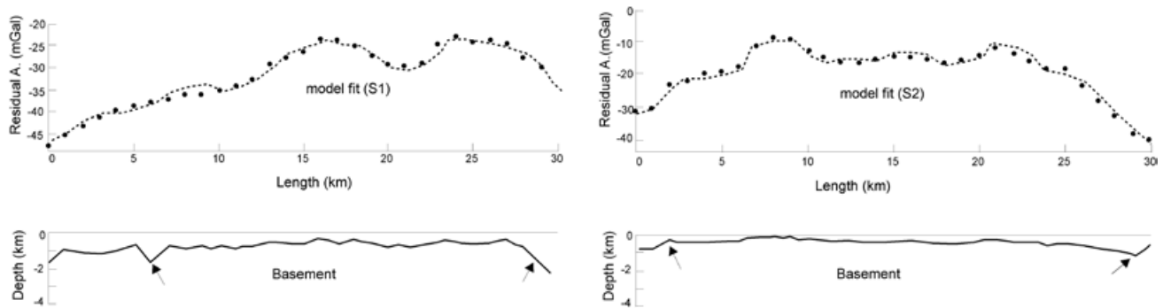
Fig. 8. Graphic of modelling sections (S1 and S2). Points represent the residual anomaly, dotted line shows the model fit, and the estimated depth is identified by the solid line below the graph. The arrows are positioned at the place of possible faults. These sections are shown in Figs. 5 and 6.
