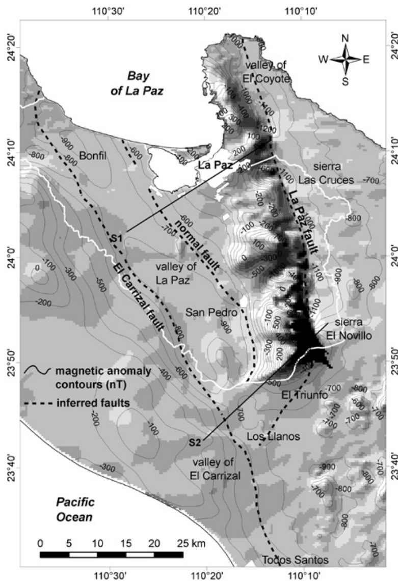
Fig. 5. Map of magnetic anomaly contours in the valley of La Paz-El Carrizal. It is shown the inferred trace of the La Paz and El Carrizal faults, an intermediate normal fault (black dotted line), the perimeter of the basin (white line polygon) and the gravity modelled sections (S1 and S2).
