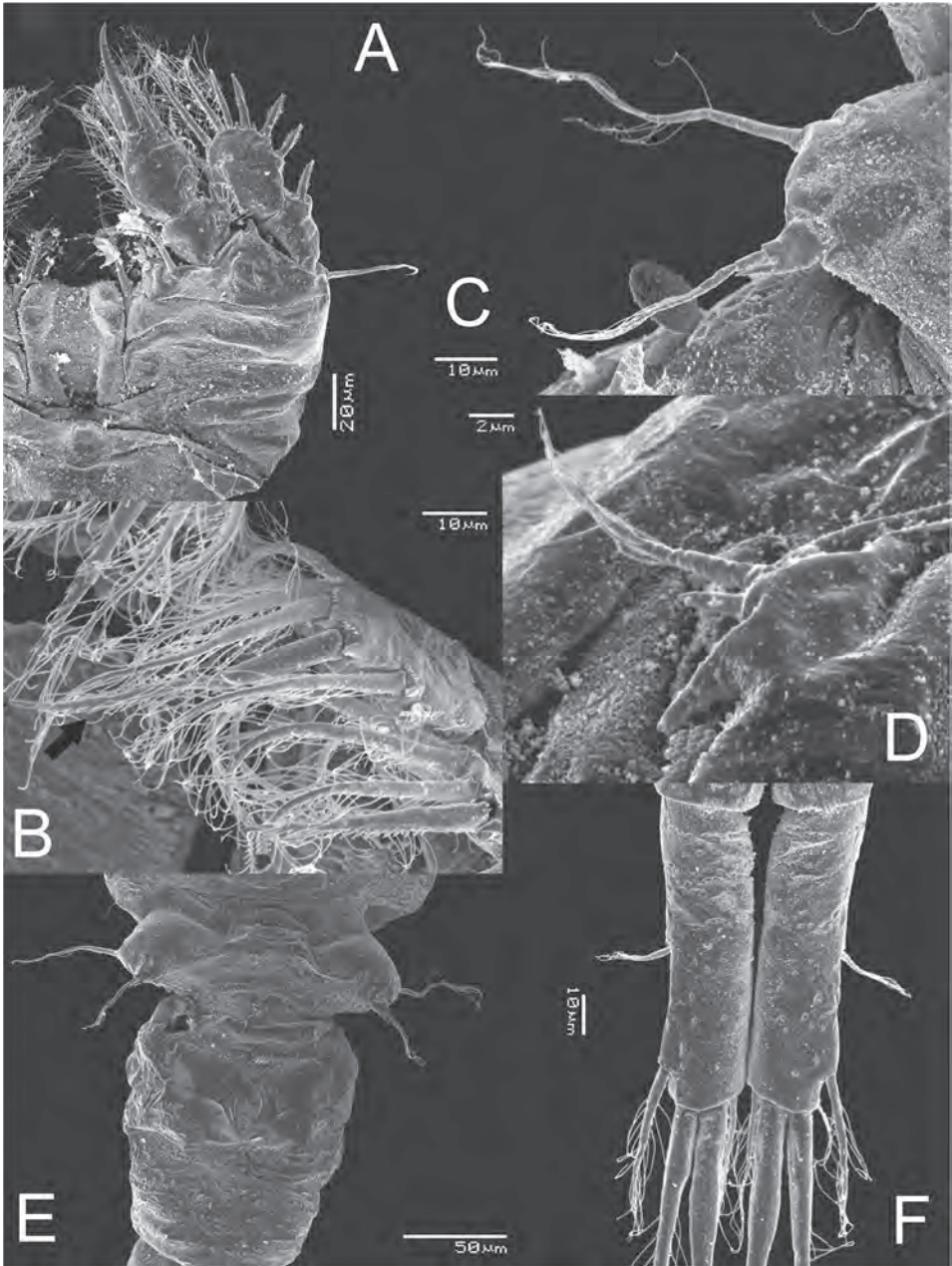
Figure 5. Metacyclops deserticus sp. n., SEM-processed female from Coahuila, México. A leg 1 B endopodite 2 leg 4 C leg 5 D leg 6 E genital double somite, ventral view F caudal ramus, ventral.
