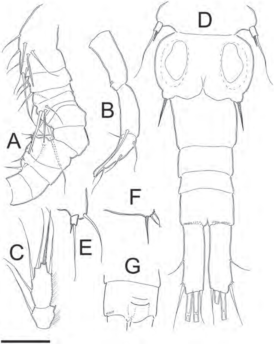
Figure 3. Metacyclops deserticus sp. n., male allotype from Coahuila, Mexico. A antennule (segments 1–11) B antennule (segments 12–14) C Endopod P4 D urosome E Leg 5 F Leg 6 G Anal operculum. Scales bars A–G = 50 \mu m.
